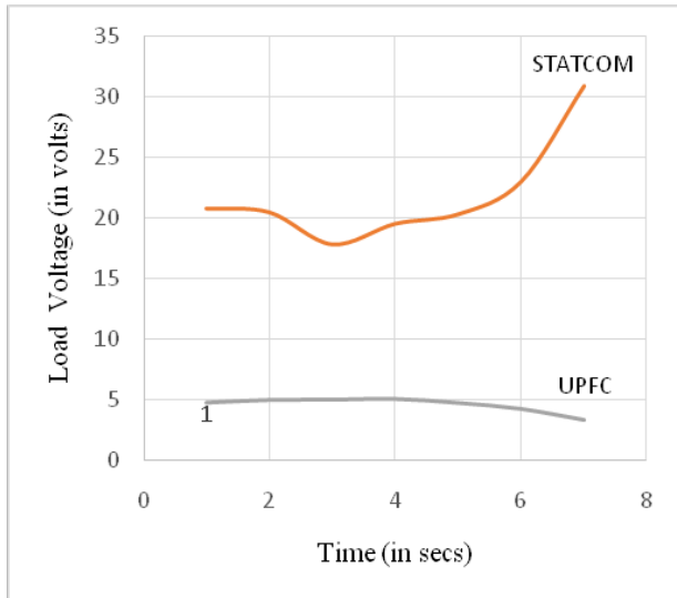
Fig. 15 - Load Voltage Characteristics with UPFC and STATCOM at Linear Load
