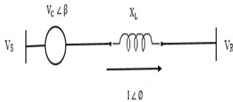
Fig 1 – Mathematical Model of UPFC
